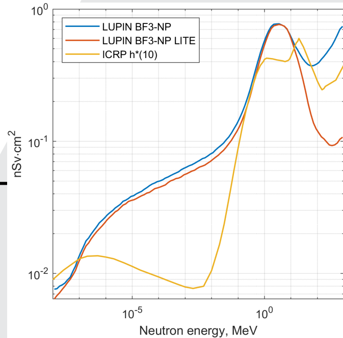
LUPIN rem counters response function VS ICRP
