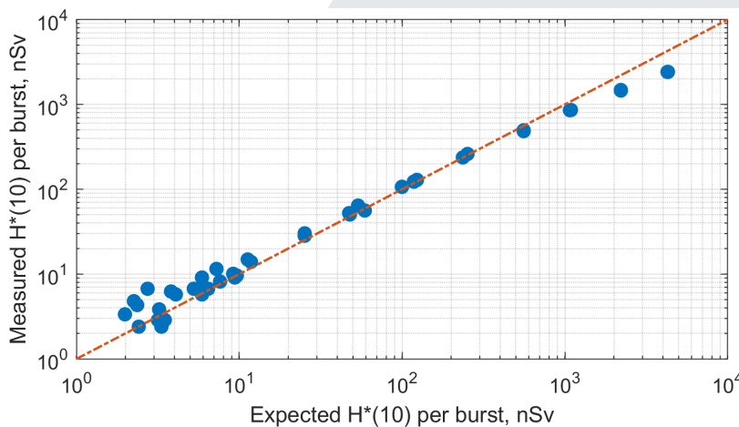
LUPIN BF3-NP performance in neutron pulsed fields
