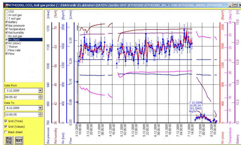
Software poCAMon
